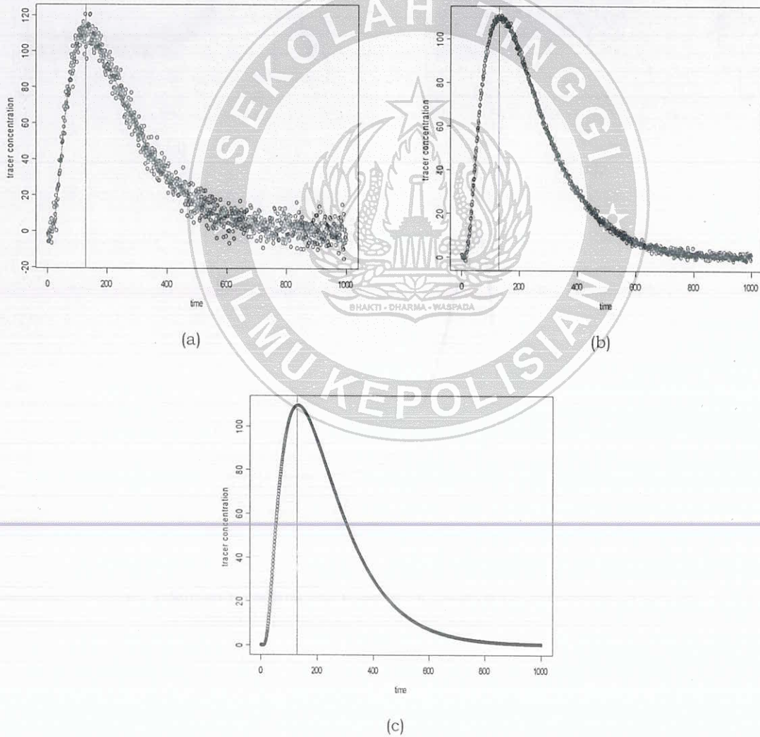
Figure 1. NLS Curve of Tracer Concentration from AH-4bis with Noise Variance: (a) 5, (b) 1, (c) 0.001
